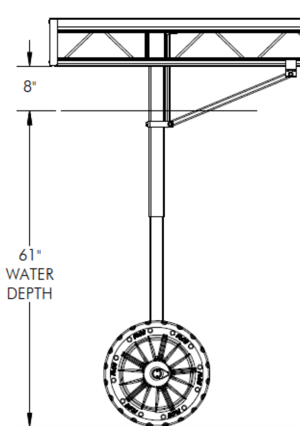
DEEP WHEEL KIT FULLY EXTENDED
