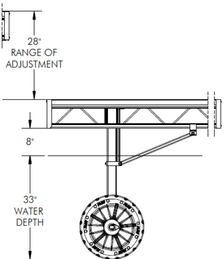
DEEP WHEEL KIT FULLY COLLAPSED
